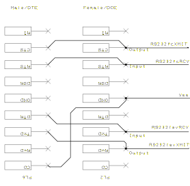
RS232 connectors
