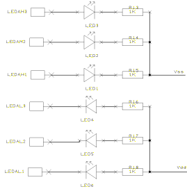
LEDs
