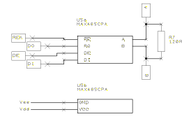
MAX485 driver
