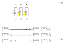
Jumpers
