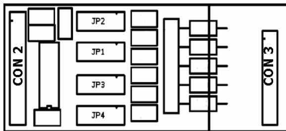
Figure 1: FLEX Multibus SPI module
