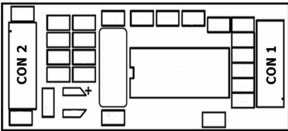
Figure 1: FLEX Multibus Ethernet module
