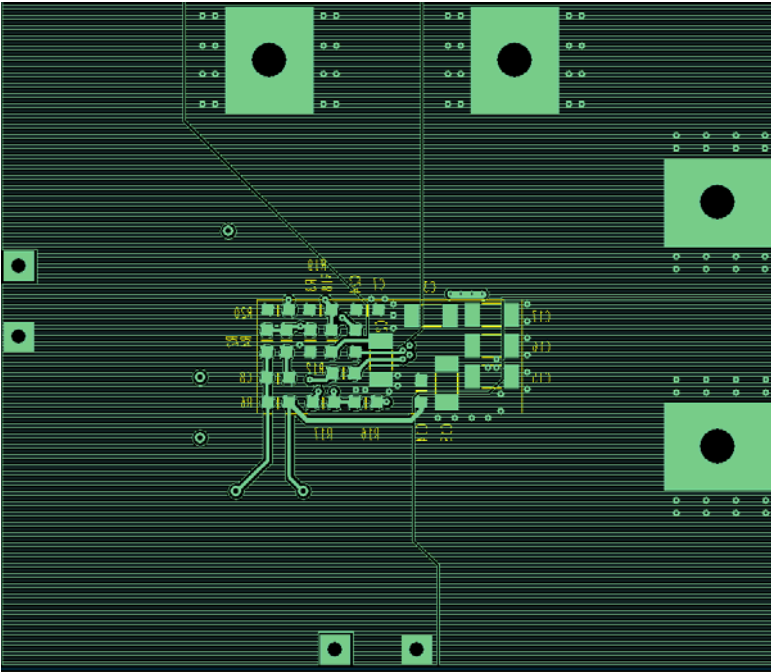
Fig. 3: Board layout, bottom overlay (rear view)
