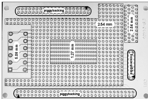
Figure 1: FLEX Thru Hole Daughter Board
