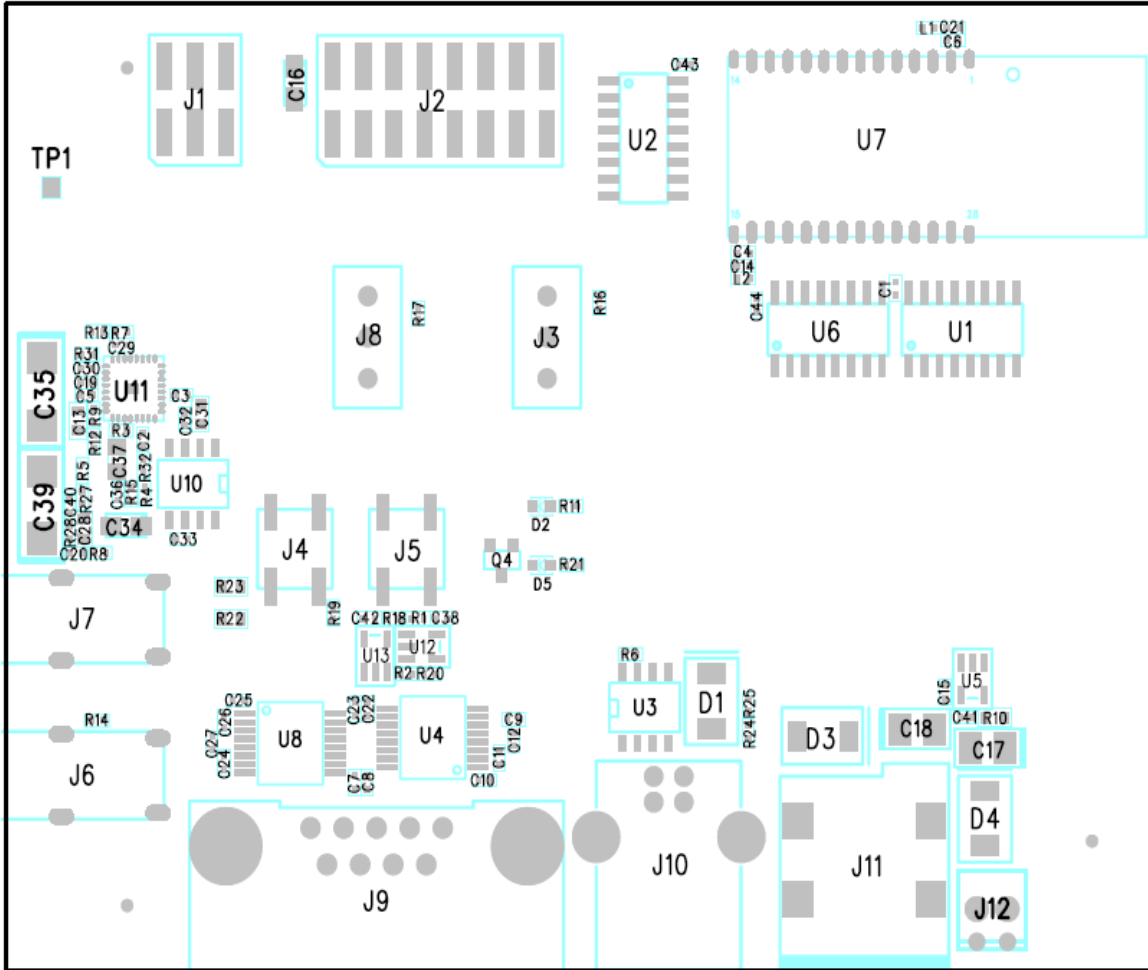
Figure 2: WT11 Evaluation Kit assembly
