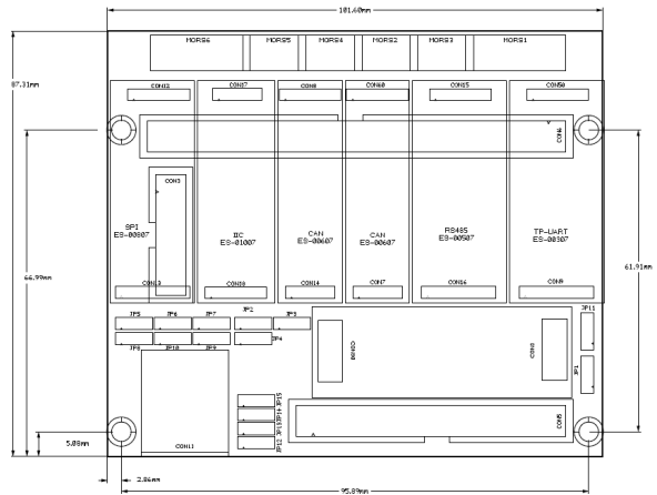
Figure 2: FLEX Multibus Base Daughter Board Dimensions
