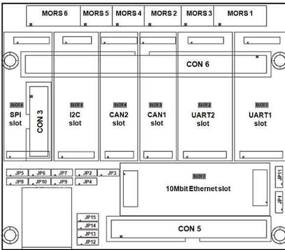
Figure 1: FLEX Multibus Base Daughter Board
