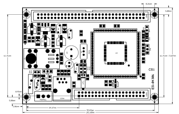
Figure 3: FLEX Light Base Board Dimensions
