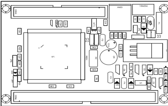
Figure 1: FLEX Light Base Board
