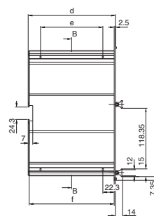
Section A – A Board depth 160 mm
