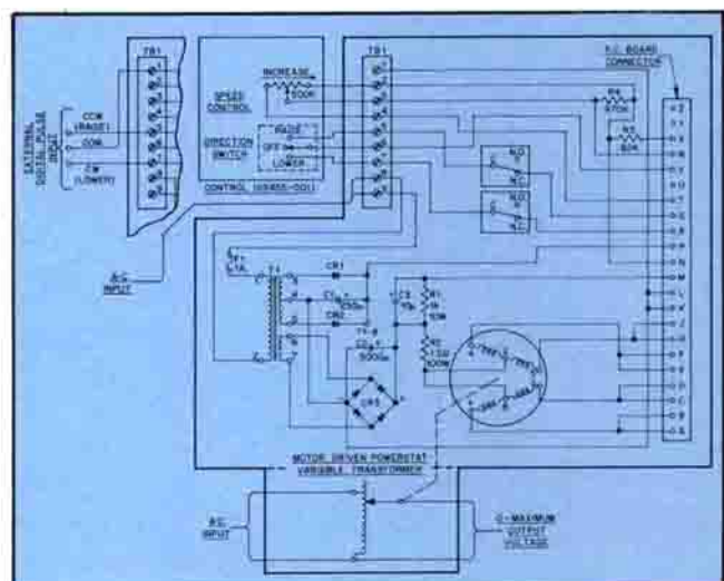
Digital Motor Drive Circuit Diagram
