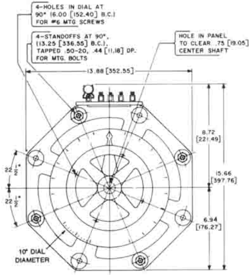
Panel Mounted
