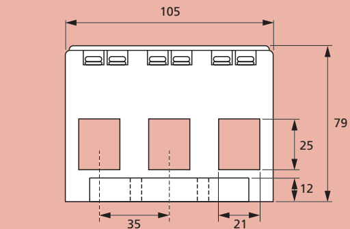
FOOT MOUNTED
