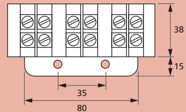
DIN RAIL MOUNTED (2 x clips supplied)
