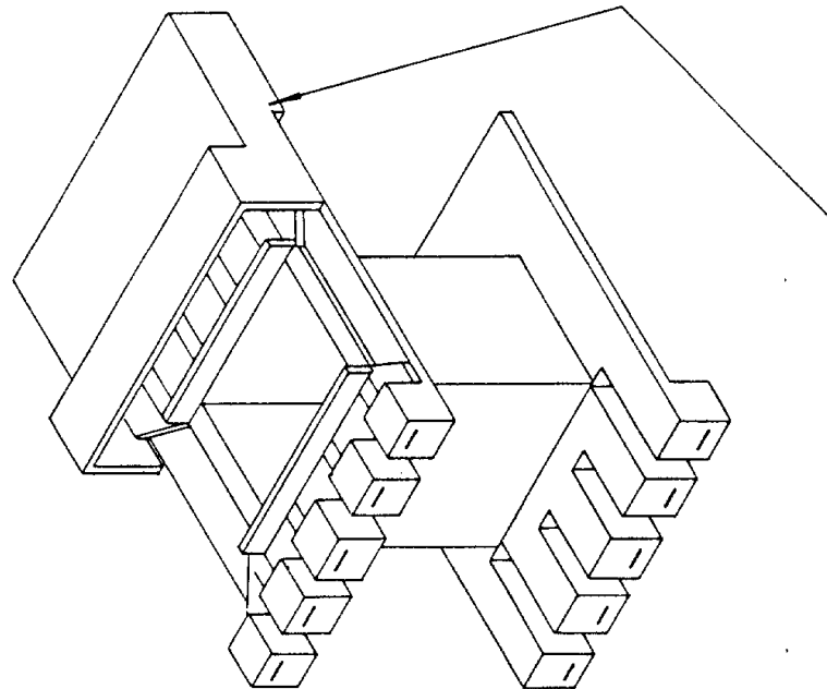
Insulator fitted to one bobbin cheek
