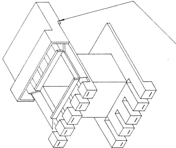
Insulator fitted to one bobbin cheek
