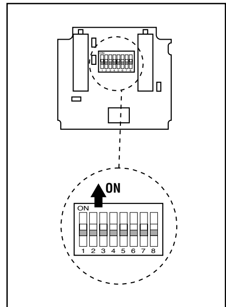
Figure 2. 45LM58 selection switch detail
