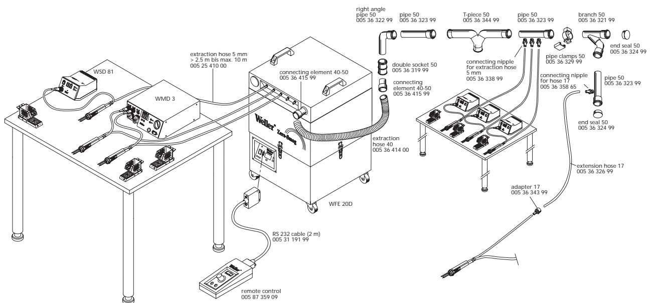
stand alone system with pipe system 50 upto ca. 200 m
