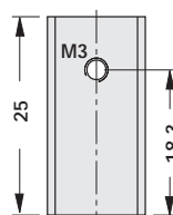
SK 95 25 TO 220
