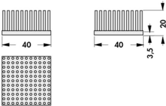
40 x 40 x 20 mm, pin heatsinks quadratic
