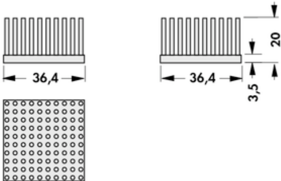
36 x 36 x 20 mm, pin heatsinks quadratic
