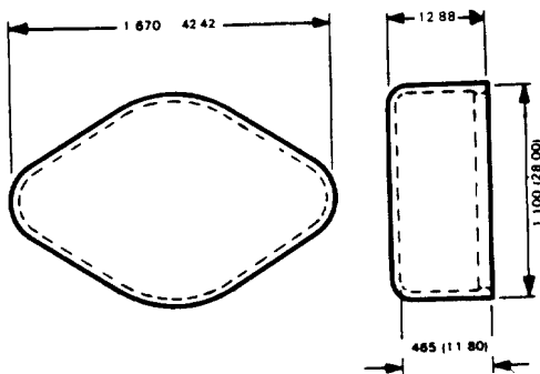
ME 416/TO 3 EXTRA HEIGHT
