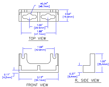
MOUNTING FEET DETAIL
