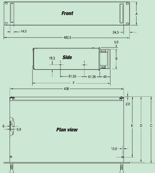
19" Rack cases
