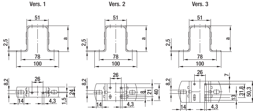
Mounting brackets for Q-motors (foot measure 26 mm)
