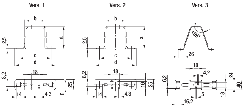
Mounting brackets for Q-motors (foot measure 18 mm)
