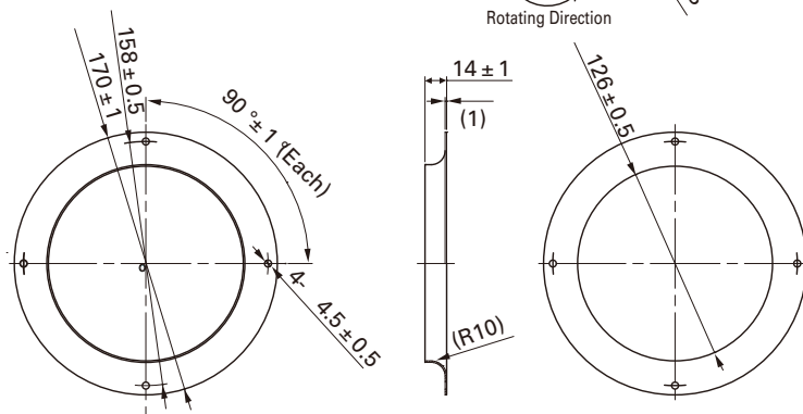
Inlet nozzle (Model : 109-1073)
