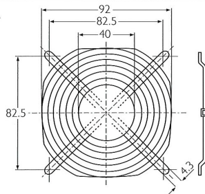
LZ23-I Rust resistant steel wire. 3xxx series fans
