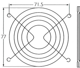
LZ22K Welded steel guard, bright nickel. 8xxx series fans
