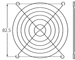
LZ23K Welded steel guard, bright zinc. 3xxx series fans
