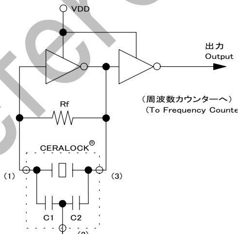
Figure 2. Test Circuit
