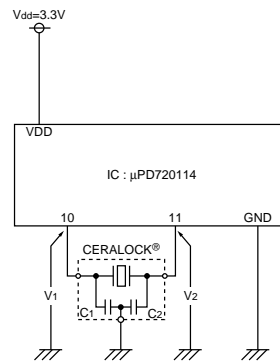
USB2.0 (Hi-speed) HUB Controller
