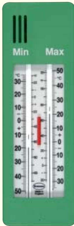
200mm Green Maximum Minimum Thermometer with black temperature scale and push button re-set.
