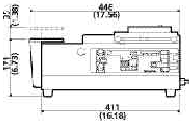
FGS-100PXH/FGS-100PXL
