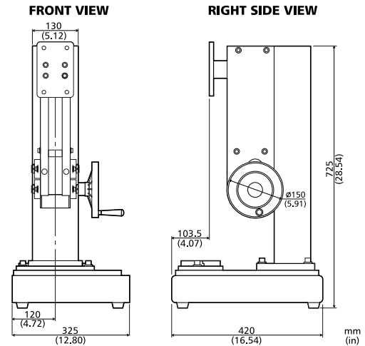
FGS-250H
