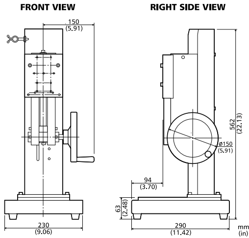
FGS-50H
