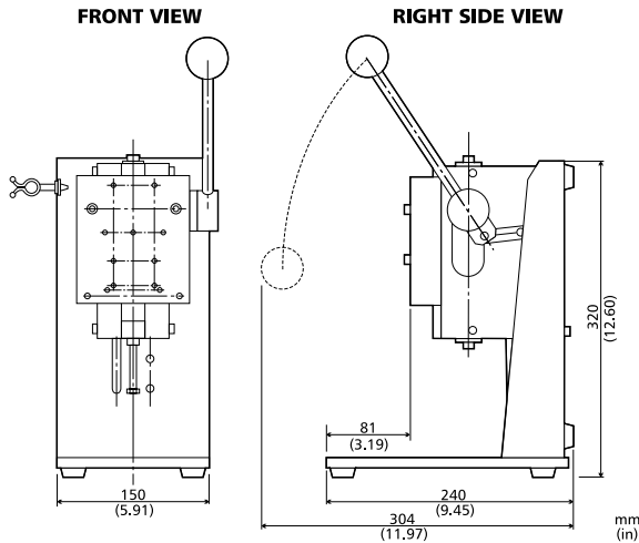
FGS-5S
