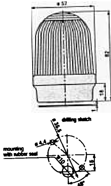
210 Permanent/LED/Flashing Beacon
