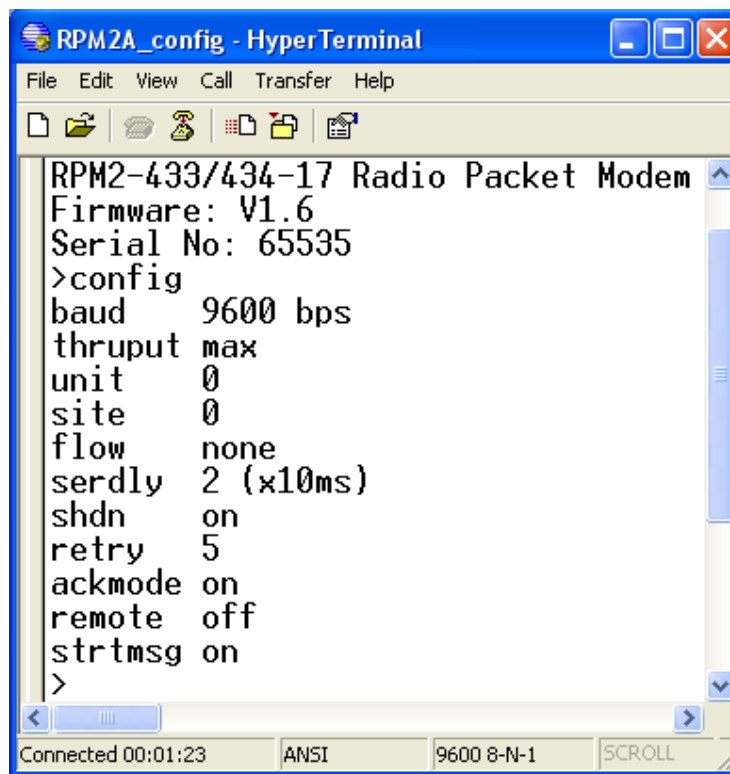
Figure 7: RPM2A configuration using HyperTerminal
