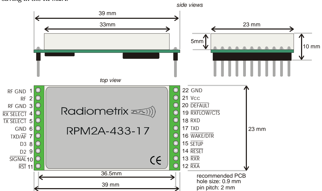
Figure 5: Physical dimensions and pinouts
