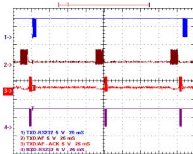
Figure 10: RPM2A operating in slots throughput mode with ACK for each transmission
