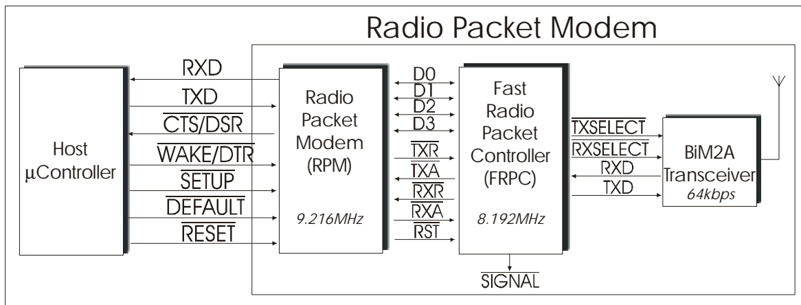
Figure 3: RPM2A block diagram
