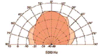
radiation pattern 5000 Hz
