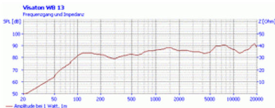
frequency response
