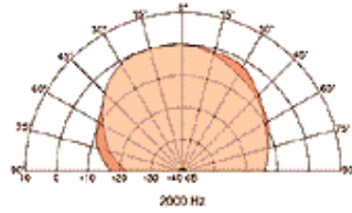
radiation pattern 2000 Hz
