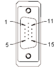
CONN2: HDB15F
