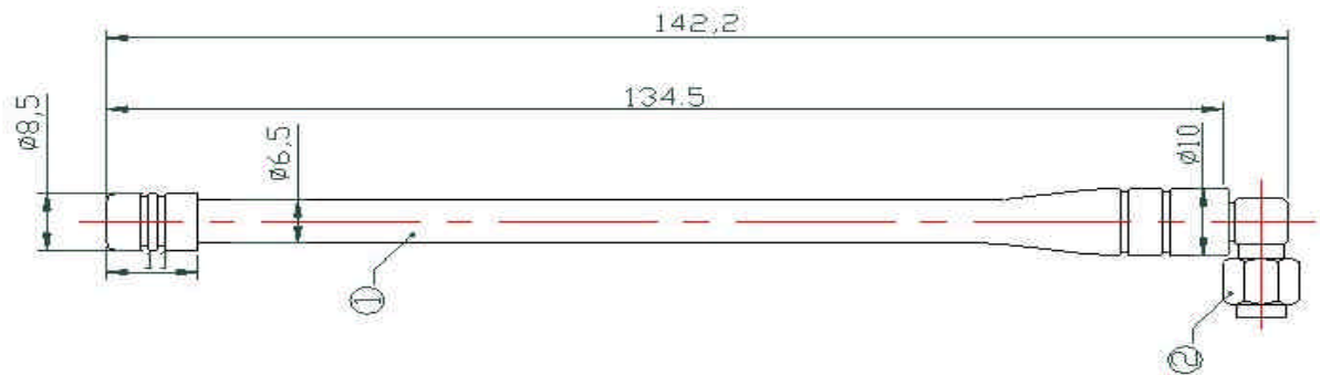
Figure 1 right-angled SMA
