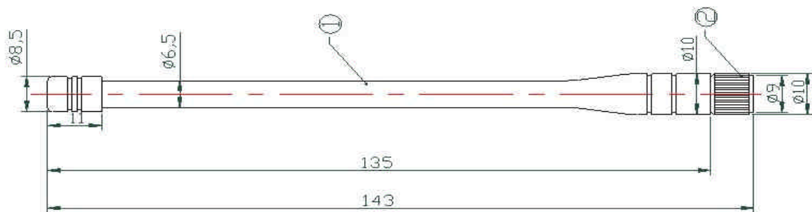
Figure 3 straight SMA
