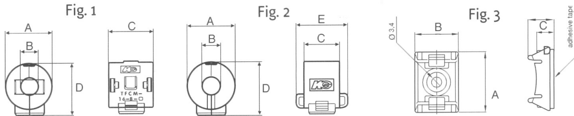
Mounting Clip
