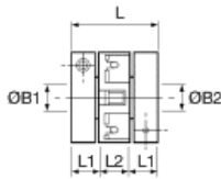
Ref. 207 Collet hub & ring clamp
