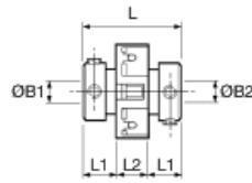
Ref. 203 Large bores
