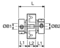
Ref. 205, 206 Integral leaf clamp
