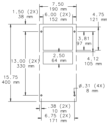
CUTOUT EXTERNAL MOUNTED
