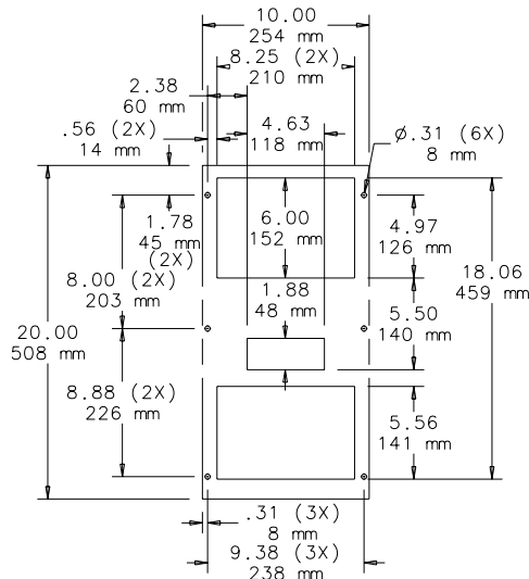
CUTOUT EXTERNAL MOUNTED
