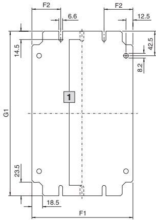
1 Attachment in the centre only for 125 mm wide plates
