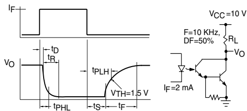
Figure 7. Saturated Switching Characteristics Measurements - Schematic and Waveform
