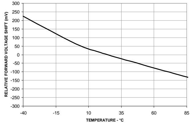
Figure 8: Temperature vs. relative forward voltage shift
