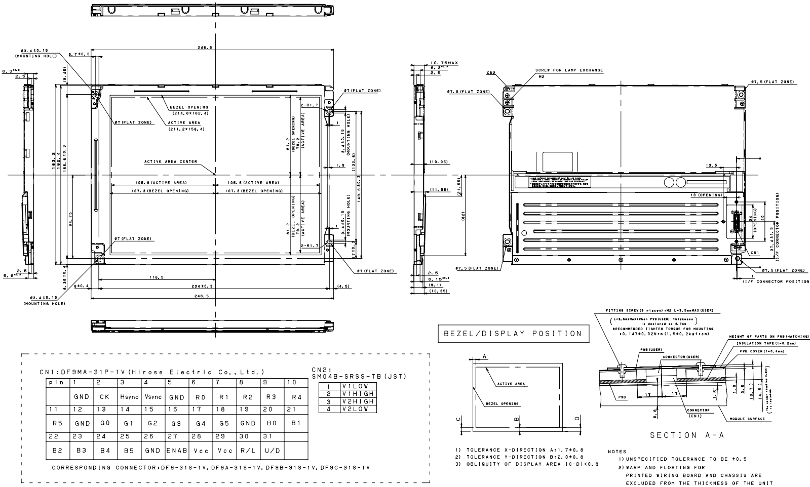
Fig1. LQ104V1DG62 OUTLINE DIMENSIONS
