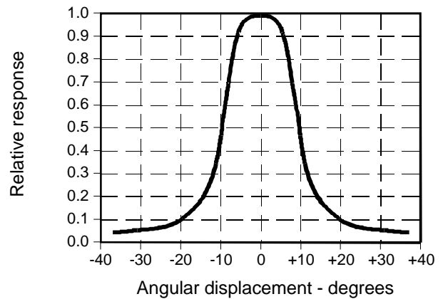
Fig. 2 Responsivity vs Angular Displacement (SD5443)
