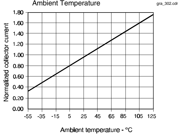
Fig. 8 Collector Current vs Ambient Temperature
