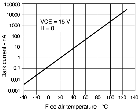
Fig. 3 Dark Current vs Temperature
