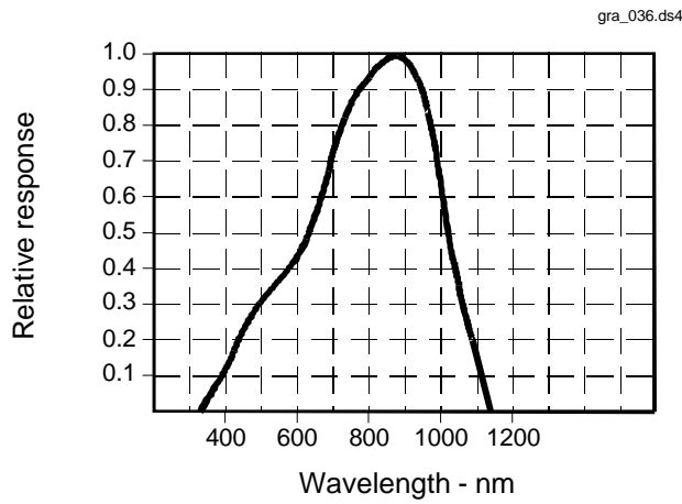
Fig. 5 Spectral Responsivity
