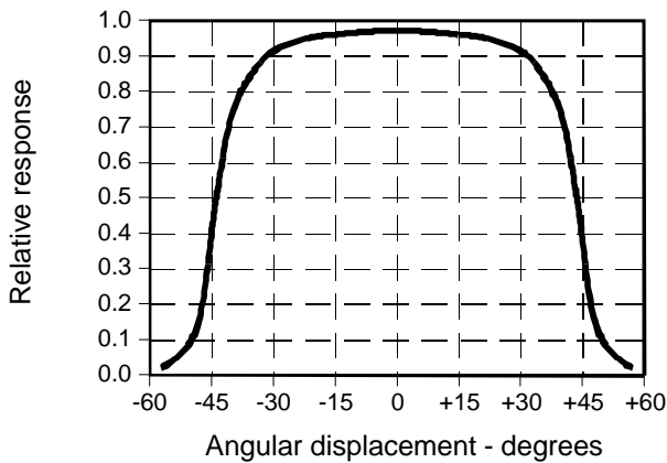
Fig. 1 Responsivity vs Angular Displacement (SD3443)
