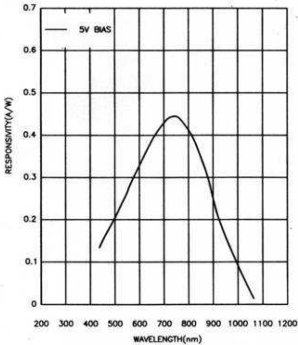
Series AEPX – Typical Spectral Response
