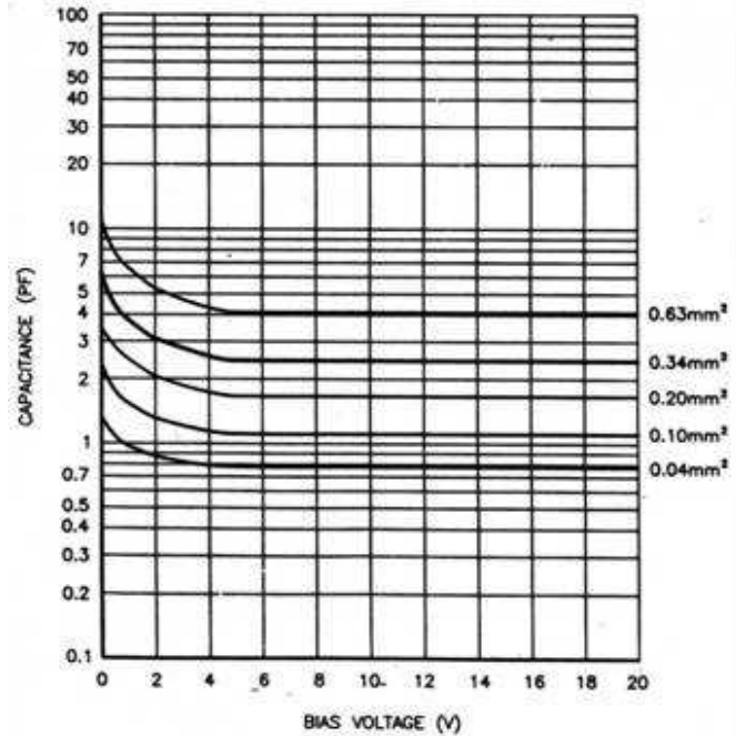
Series AEPX – Typical Capacitance versus Bias Voltage
