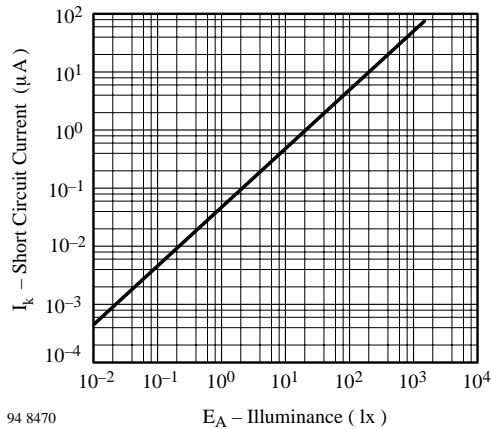
Figure 3. Short Circuit Current vs. Illuminance
