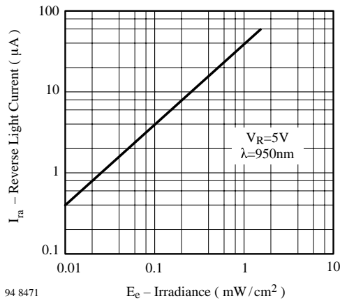
Figure 4. Reverse Light Current vs. Irradiance
