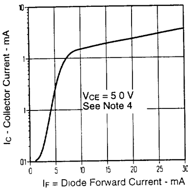
Collector Current vs Diode Forward Current
