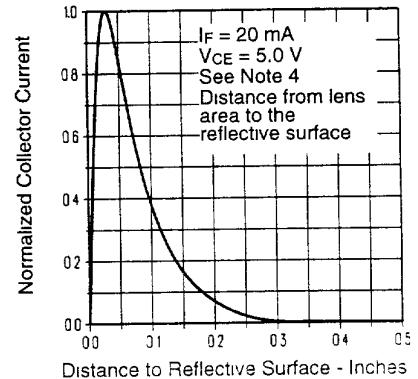
Normalized Collector Current vs Object Distance
