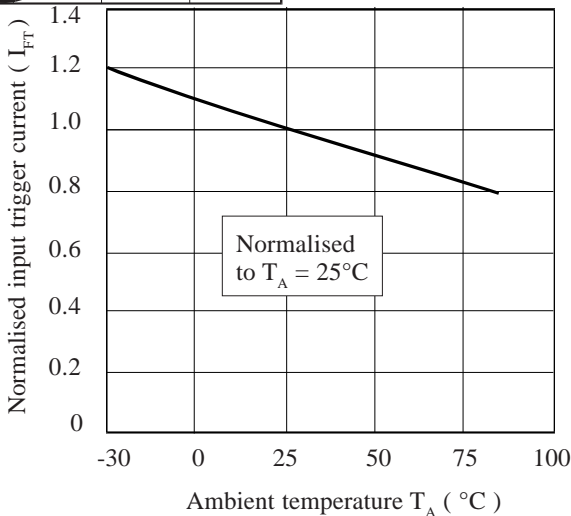
Normalised Input Trigger Current vs. Ambient Temperature
