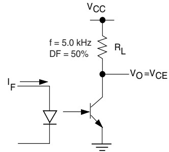
Fig. 6 Switching Schematic
