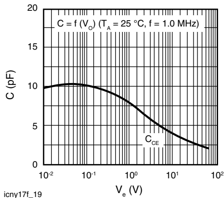
Fig. 19 - Transistor Capacitance
