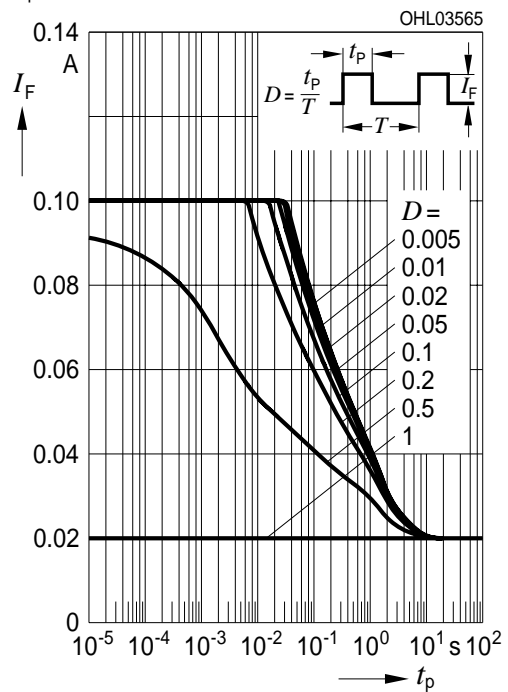
Zulässige Impulsbelastbarkeit Permissible Pulse Handling Capability Duty cycle D = \text{parameter} , T_A = 85^\circ\text{C} I_F = f(t_p) ; red (3 Chips on)
