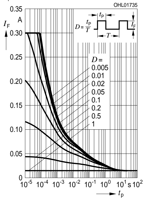
Zulässige Impulsbelastbarkeit Permissible Pulse Handling Capability Duty cycle D = \text{parameter} , T_A = 85\text{ °C} I_F = f(t_p) ; blue (3 Chips on)
