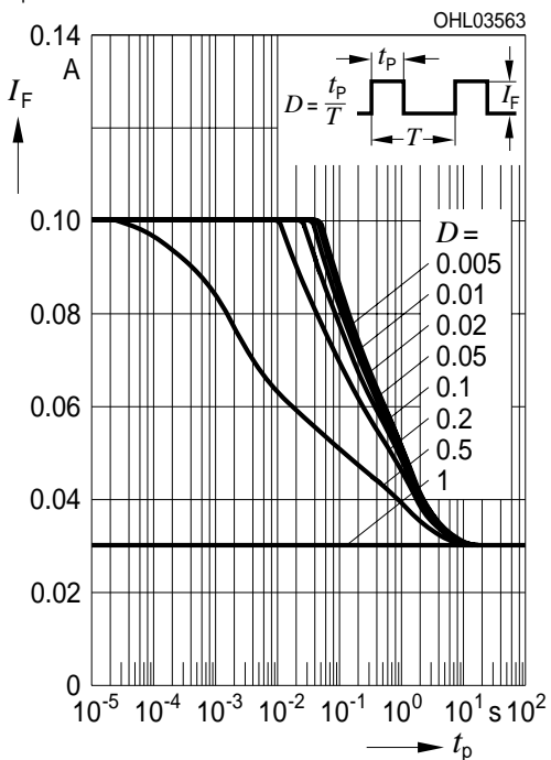
Zulässige Impulsbelastbarkeit Permissible Pulse Handling Capability Duty cycle D = \text{parameter} , T_A = 85^\circ\text{C} I_F = f(t_p) ; red (1 Chip on)
