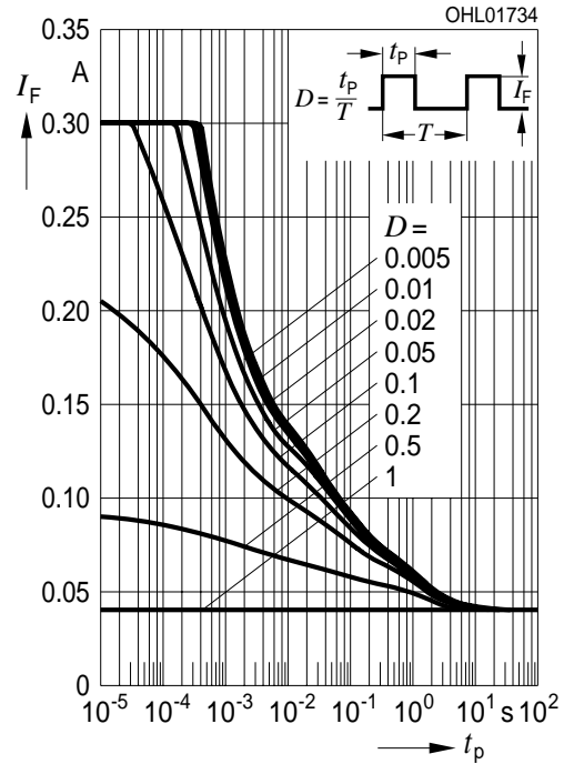
Zulässige Impulsbelastbarkeit Permissible Pulse Handling Capability Duty cycle D = \text{parameter} , T_A = 85\text{ }^\circ\text{C} I_F = f(t_p) ; true green (3 Chips on)
