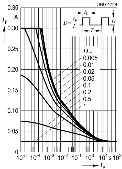
Zulässige Impulsbelastbarkeit Permissible Pulse Handling Capability Duty cycle D = \text{parameter} , T_A = 85\text{ }^\circ\text{C} I_F = f(t_p) ; true green (1 Chip on)
