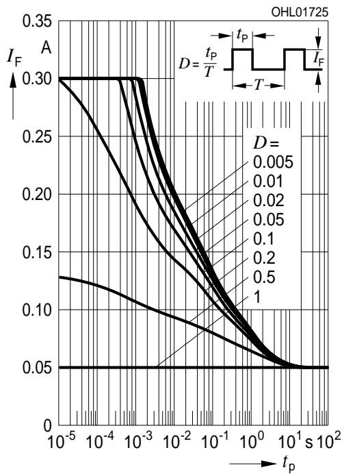
Zulässige Impulsbelastbarkeit Permissible Pulse Handling Capability Duty cycle D = \text{parameter} , T_A = 85\text{ °C} I_F = f(t_p) ; blue (1 Chip on)
